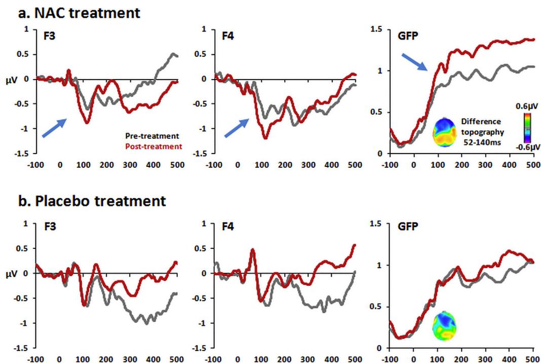
Fig. 2. Group-averaged voltage waveforms from frontal sites F3 and F4 as well as GFP waveforms from patients who received NAC and placebo treatment (panels A and B, respectively). Gray traces display responses pre-treatment and red traces responses post-treatment. Insets display the difference topography averaged over the 52–140 ms period. Blue arrows indicate the significant differences before and after NAC treatment over the N100 period. (For interpretation of the references to color in this figure legend, the reader is referred to the web version of this article.)
