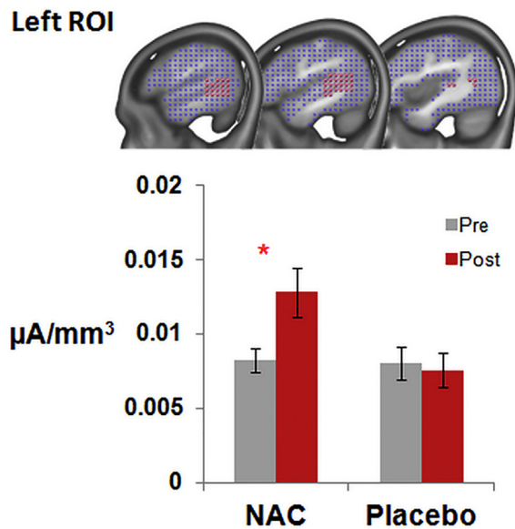
Fig. 3. Results of the mixed ANOVA on the mean source activity on the predefined left temporal cortex region. Asterisks indicate significant differences between pre and post-treatment for the patients that received NAC. Source activity was estimated on data averaged over the 52–140 ms period. Inset indicates the selected points for the left hemisphere (pink nodes). A symmetric set of points was tested in the right hemisphere. (For interpretation of the references to color in this figure legend, the reader is referred to the web version of this article.)
