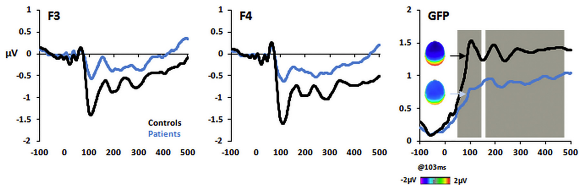
Fig. 1. Group-averaged voltage waveforms from frontal sites F3 and F4 as well as global field power (GFP) waveforms from control subjects and early psychosis patients (black and blue traces, respectively). The gray areas in the GFP waveforms indicate significant differences as a function of time. Responses were weaker in patients. (For interpretation of the references to color in this figure legend, the reader is referred to the web version of this article.)
